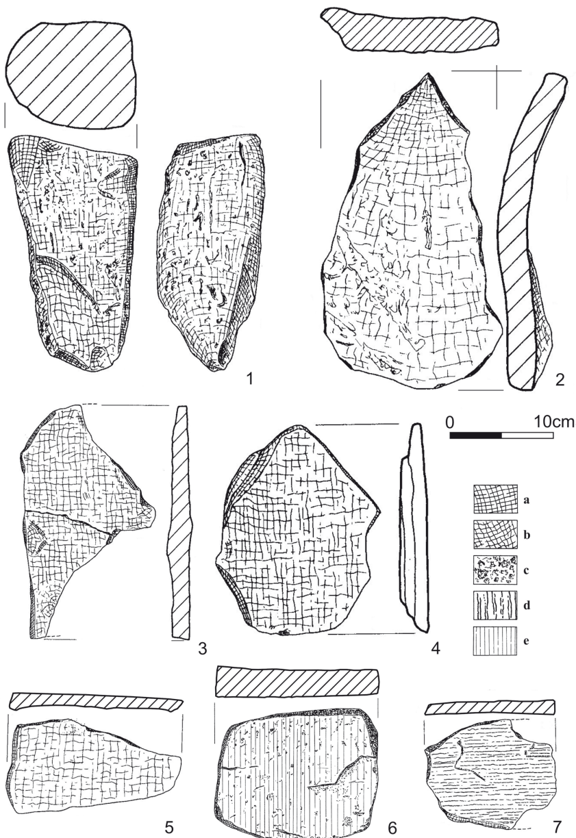
Fig. 2. Stone products of GAC population (drawings by P. Chachlikowski, J. Wierzbicki). Detailed information on the sites where individual products were unearthed as well as their chronology are shown in Tables 1 and 2. 1 – unfinished (initial) form of adze; 2-5 – unfinished forms (semi-products) of polishing plates; 6 – polishing plate; 7 – fragment of a polishing plate. Raw materials: gneiss – 1; quartzite – 3, 4; quartzitic sandstone – 2, 5-7. Key: a – natural surface; b – negative surface; c – breaks; d – surface with traces of stripping (grinding); e – surface with traces of polishing
